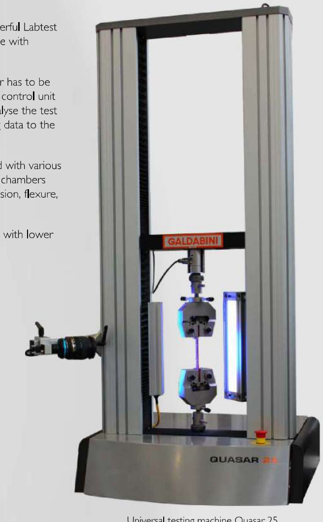
Universal testing machine Quasar 25 with Video extensometer
